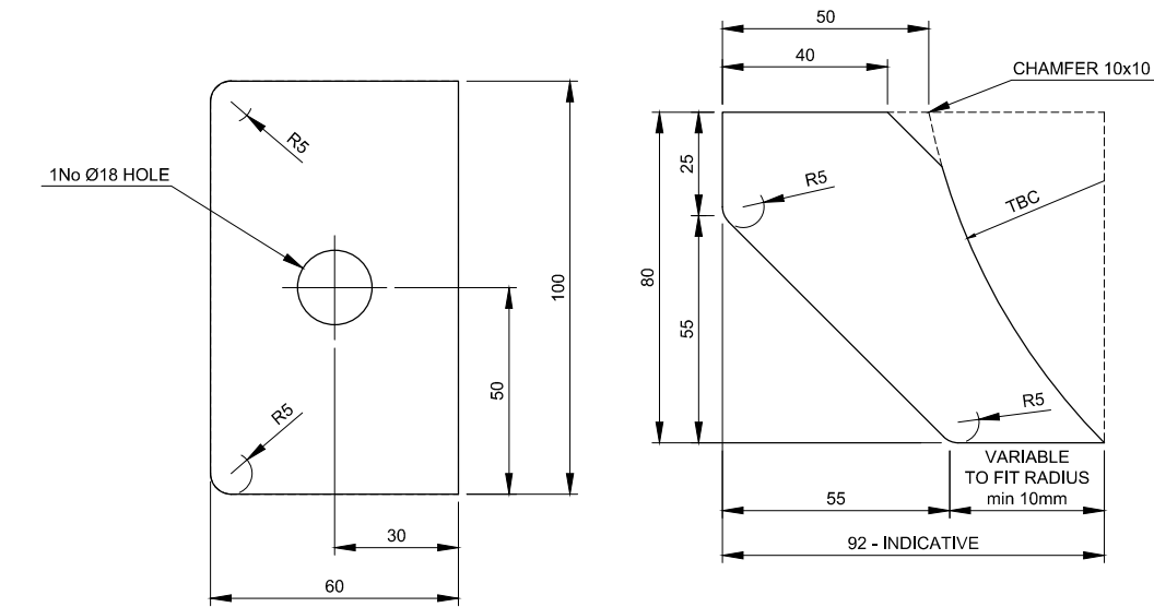
TPC-A-1 - 15mm THICK Scale 1:2
