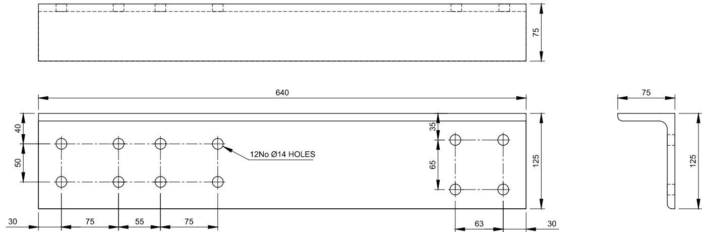
TPA-V - UA125x75x10 Scale 1:5
