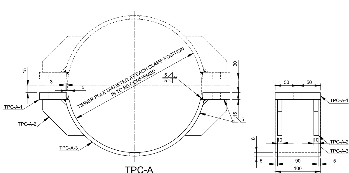
TPC-A Scale 1:5
