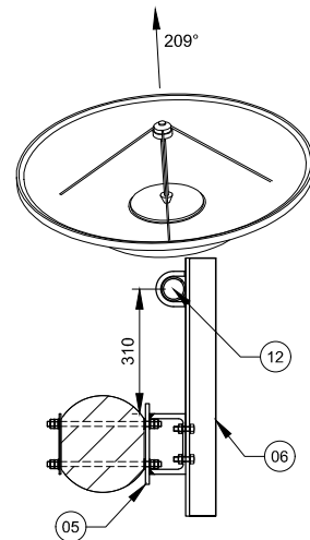
SECTION D-D Scale 1:20
