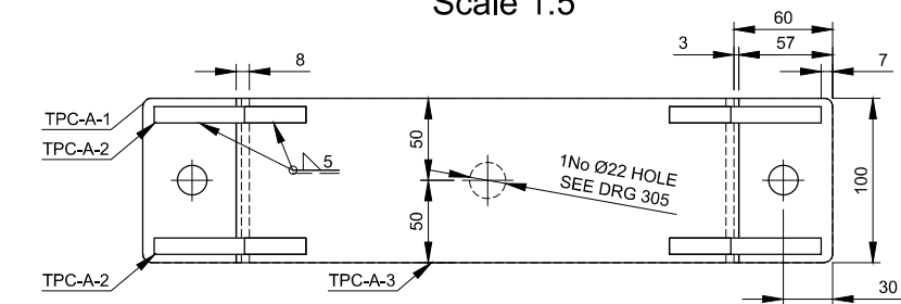
TPC-A Scale 1:5
