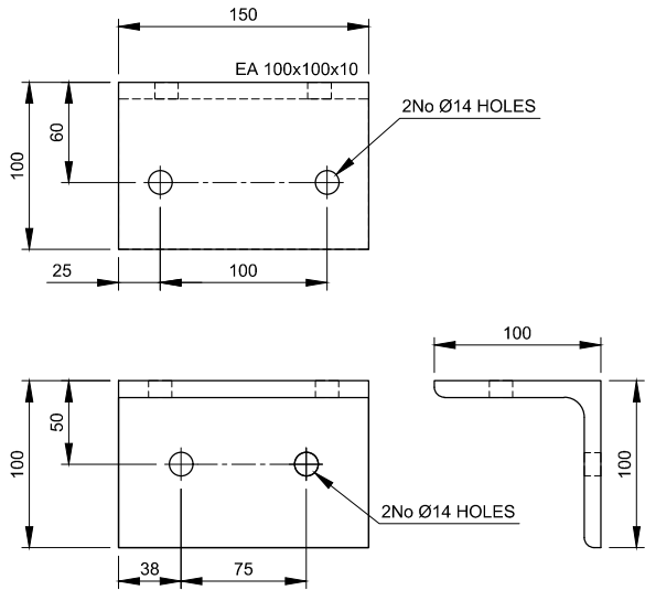
TPL-A - EA100x100x10 Scale 1:5
