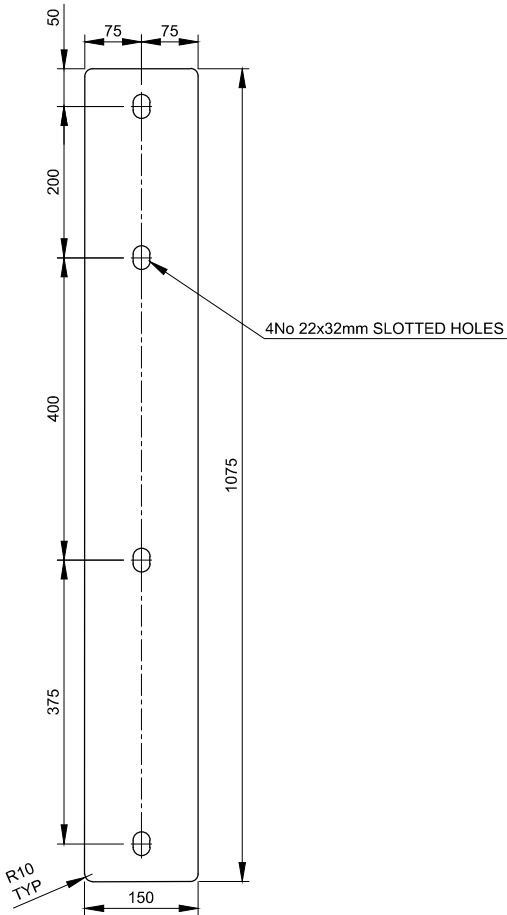
TPC-B - 15mm THICK Scale 1:10
