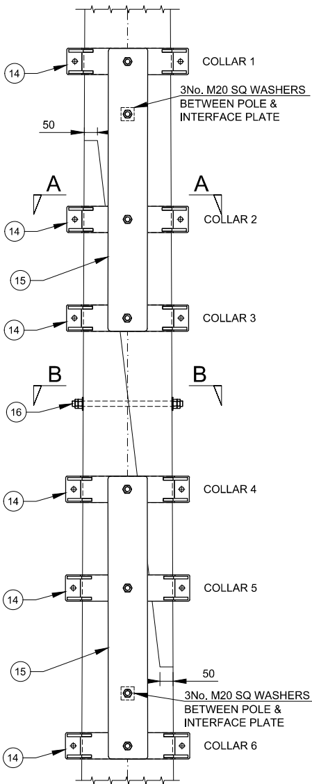
DETAIL I TIMBER POLE SPLICE Scale 1:20
