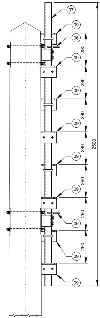
SECTION C-C Scale 1:20
