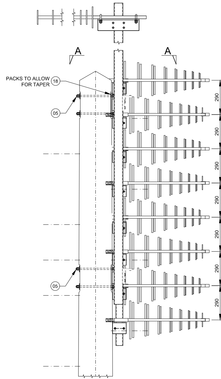
DETAIL G - Rx & Tx ANTENNA MOUNTS Scale 1:20
